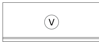
OS00457 301x120x12mm
