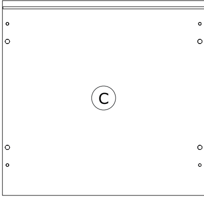
CA04222 367x353x16mm
