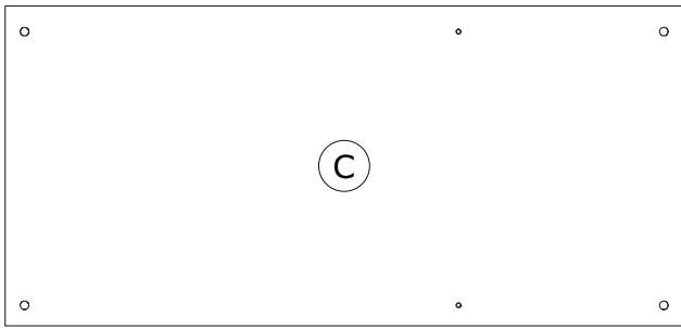
PI07935 1189x561x16mm
